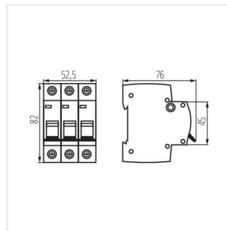
KMB6-B32/3
