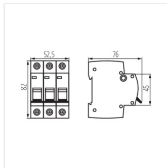
KMB6-B16/3
