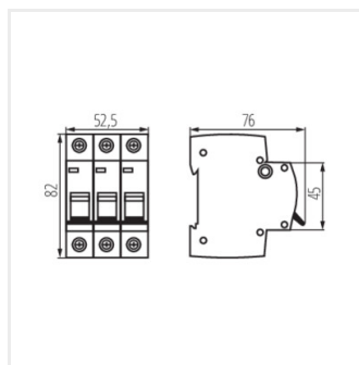
KMB6-B50/3
