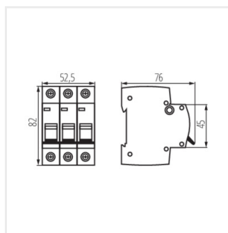
KMB6-B40/3
