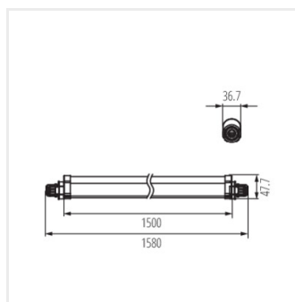
TP_SLIM_N-TN 50W
