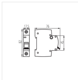
KMB10-C2/1
