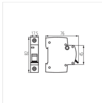
KMB10-C63/1
