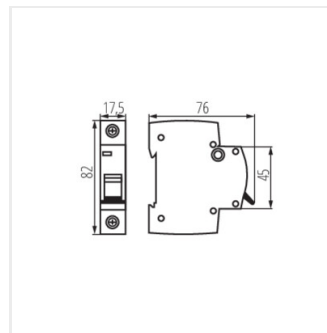
KMB10-C13/1
