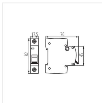
KMB10-C4/1
