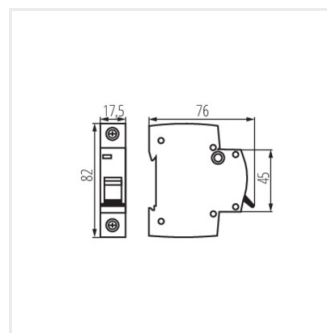
KMB10-C50/1
