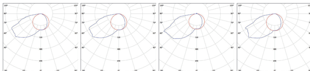
MAGION LED Emergency 180min 5,6W under mains power
